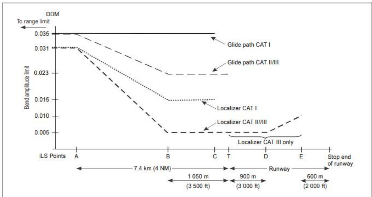
Figure C-1. Localizer course and glide path bend amplitude limits
